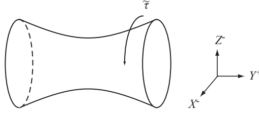
Fig. 6.2 The embedding of \text{AdS}_2 into \mathbb{R}^{2,1} . The timelike direction \tilde{\tau} is periodic, so we consider the covering space.
