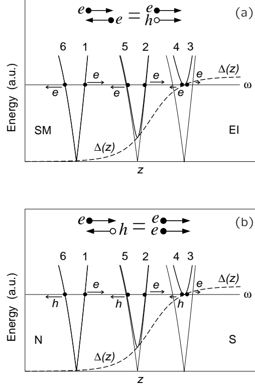
Fig. 1.2 Andreev reflection. (a) SM-EI junction. An incoming b -band electron is backscattered into the a band. The thicker (thinner) curves are the renormalized (bare) bands at different values of the z coordinate, with \Delta(z) being the corresponding order parameter. Only the relevant low-energy portion of the spectrum is shown here, with numbers from 1 to 6 pointing to the time sequence of the reflection process (the arrows represent group velocities). The inset illustrates that the reflection process may alternatively be seen as a coherent flow of excitons from the SM into the EI. (b) N-S junction. In contrast to panel a, an electron is backscattered as a hole, hence the whole process may be thought of as the dissipationless flow of Cooper pairs through the interface.
