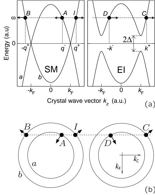
Fig. 1.1 Junction between semimetal (SM, left) and excitonic insulator (EI, right). (a) Quasi-particle energy \omega vs wave vector k_z . The labels mark the allowed elastic scattering channels for an incoming electron (labeled I ) with k_z = q^+ . In particular, A is the interband (Andreev) reflection, B the intraband reflection, C the intraband transmission, and D the interband transmission. The size of the EI gap is 2\Delta . (b) Isoenergetic contour lines in the (k_x, k_z) space for the energy \omega shown in panel a. The arrows point to the group velocities of electrons in the different scattering channels.
