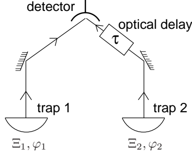
Fig. 1.9 Proposed experimental setup to measure the time correlation of the photons emitted from the two traps. The delay time \tau of one optical path is externally controlled.
