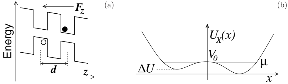
Fig. 1.8 (a) Double quantum well energy profile along the growth direction z . Electrons and hole move freely in the xy planes at z = d and z = 0 , respectively. F_z is the component of the electric field parallel to the exciton electric dipole. (b) Effective exciton potential profile vs x for the double-trap setup.
