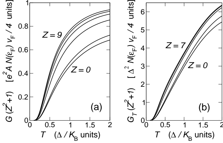
Fig. 1.6 (a) Electrical conductance G of the SM-EI junction vs temperature T . The curves correspond to different values of the dimensionless barrier opacity, Z = 0, 1, 3, 5, 7, 9 . For each value of Z , G is divided by the corresponding transmission coefficient when \Delta = 0 , i.e., C_{\Delta=0} = (Z^2 + 1)^{-1} . K_B is the Boltzmann constant, A is the interface cross-sectional area, N(\epsilon_F) is the density of states evaluated at the Fermi energy \epsilon_F . (b) Thermal conductance G_T of the SM-EI junction vs T . The curves correspond to Z = 0, 1, 3, 5, 7 .
