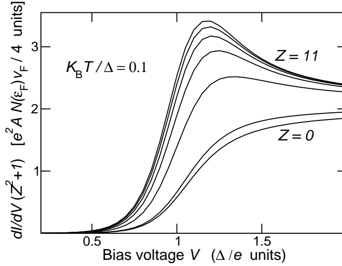
Fig. 1.7 Differential conductance (dI/dV)/C_{\Delta=0} of the SM-EI junction vs bias voltage V , computed at K_B T/\Delta = 0.1 . The curves correspond to different values of the dimensionless barrier opacity, Z = 0, 1, 3, 5, 7, 9, 11 . For each value of Z , dI/dV is divided by the corresponding transmission coefficient when \Delta = 0 , i.e., C_{\Delta=0} = (Z^2 + 1)^{-1} .
