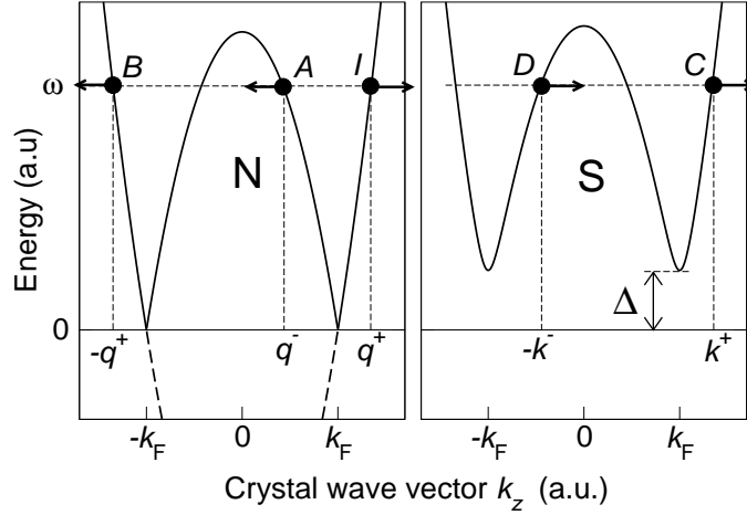
Fig. 1.3 Junction between normal metal (N, left) and superconductor (S, right). The plot shows the quasiparticle energy \omega vs wave vector k_z in the two bulk phases. The labels mark the allowed elastic scattering channels for an incoming particle (labeled I ) with k_z = q^+ . A is the Andreev reflection, B the normal reflection, C the normal transmission, and D the cross-branch transmission. Note that the energy of the particle is positive: on the N side the hole branch for |k_z| < k_F is obtained by inverting the energy of the portion of band filled with electrons (showed as a dashed curve) with respect to the Fermi surface.
