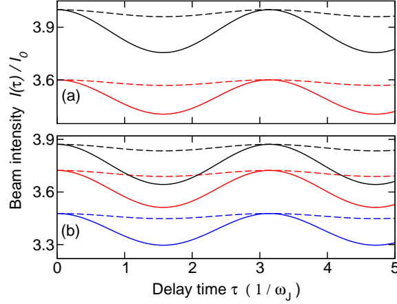
Fig. 1.10 (Color online). Beam intensity I(\tau)/I_0 vs delay time \tau , for \Delta U/\hbar\omega_J = 0.2, 0.5 (dashed and solid lines, respectively). (a) T = 0 and \alpha = 1, 0.8 (black and red [light gray] lines, respectively). (b) \alpha(T = 0) = 0.94 and k_B T/\hbar\omega_J = 0, 1, 2 (black, red [light gray], and blue [dark gray] lines, respectively).
