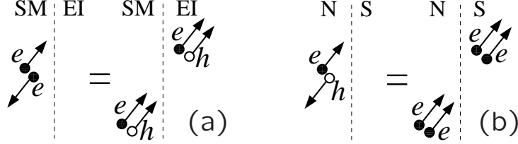
Fig. 1.4 Sketch of Andreev reflection for quasiparticles approaching the junction from the normal-phase side. (a) SM-EI junction. The reflected left-going electron is equivalent to a right-going hole. (b) N-S junction. The reflected left-going hole is equivalent to a right-going electron.
