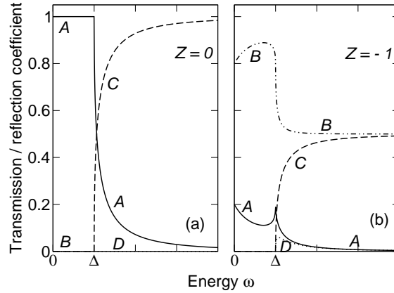
Fig. 1.5 Transmission and reflection coefficients at the SM-EI boundary vs quasiparticle energy \omega . (a) Z = 0 . (b) Z = -1 . A gives the probability of Andreev reflection, B gives the probability of ordinary reflection, C gives the transmission probability without branch crossing, and D gives the probability of transmission with branch crossing. The parameter Z measures the interface transparency.
