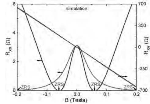
Fig. 2: Simulations of R_{xx} vs. B identify a zero-resistance state (ZRS) at a finite B resulting from the bell-shape negative magnetoresistance. Here, the traces in red present a simulation in an effective two-conduction model where R_{xx} \rightarrow 0 in the high- B limit. The traces in blue examine a three-conduction model which includes positive magnetoresistance in the high B -limit. Here, a zero-resistance state appears possible over a narrow B interval, in the vicinity of B=0.06 Tesla.
