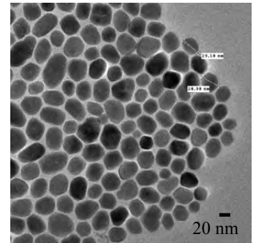
Fig. 1: TEM image of Fe-ITO NPs with 1.0% Fe and 2.1% Sn.
