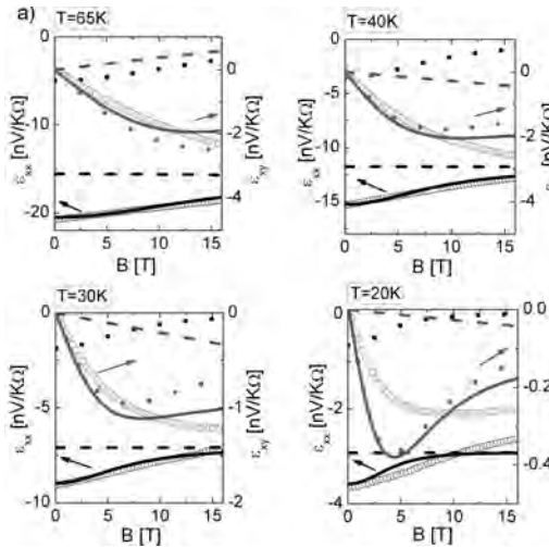
Fig. 2: \varepsilon_{xx} (left side, black) and \varepsilon_{xy} (right side, gray) for selected temperatures. Measured data (open symbols), fit with the two-charge-carrier model (lines) and con-tribution of the two charge carriers ( n_1; \mu_1 ), ( n_2; \mu_2 ) respectively (dashed and dotted lines).
