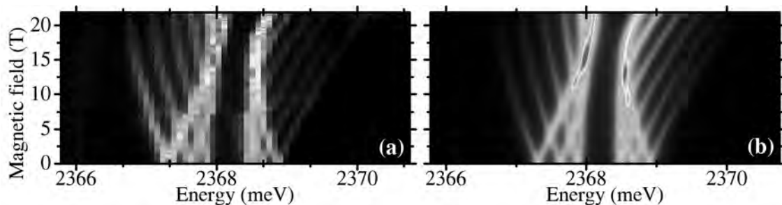
Fig. 1: (a) Experimental and (b) simulated PL spectrum of an exciton in a CdSe/ZnSe QD with a single \text{Mn}^{2+} ion as a function of magnetic field in Faraday configuration.
