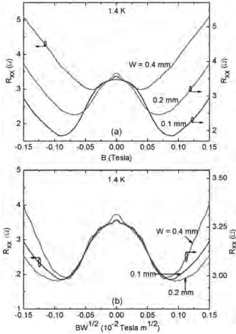
Fig. 1 (a) This panel compares the R_{xx} vs. B for W = 0.4, 0.2 , and 0.1 mm sections of a variable width Hall bar at 1.4 K. The panel suggests a monotonic increase in the full-width at half-maximum of the "bell-shape" magnetoresistance, with decreasing W . (b) At 1.4 K, R_{xx} has been plotted vs. BW^{1/2} in order to convey the size scaling of the "bell-shape" magnetoresistance observed for W = 0.4, 0.2 , and 0.1 mm-
