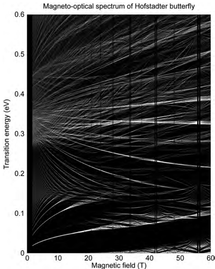
Fig. 1: Intensity map of optical conductivity for right circularly polarized light of twisted bilayer graphene with \theta = 2.65^\circ . Magneto-optic spectrum evolves into a fractal [6].
