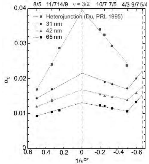
Fig. 1: The measured critical values of E_Z/(e^2/4\pi\epsilon l_B) above which the CFs at a given CF filling factor n^{CF} become fully spin-polarized, \alpha_c , is plotted as a function of 1/n^{CF} ; the electron filling factors are given in the top axis. Dotted lines are guides to the eye and represent the phase boundary above which the CFs become fully spin-polarized for each quantum well width.
