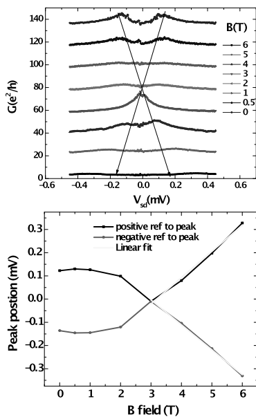
Fig. 1: a) The magnetic field dependence of the conductance G(V) normalized to zero field conductance without Kondo effect, G_0(V) . At 3 T, close to B_{ST} , we observed a zero-bias conductance enhancement. b) Cotunneling features vs B . This result may indicate a possible observation of the 2-ch Kondo effect under the dissipative environment.
