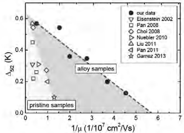
Fig. 1: The dependence of the energy gap \Delta_{5/2} of the \nu=5/2 fractional quantum Hall state on inverse mobility 1/\mu of our samples (closed symbols) and of alloy-free samples from the literature with densities near 2.9 \times 10^{11}/\text{cm}^2 . In our alloy samples the \nu=5/2 fractional state survives at surprisingly high 1/\mu and, therefore, low \mu .
