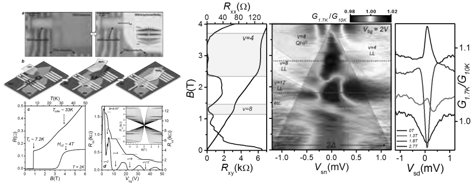
Fig. 1. a) +b) Optical image of the device and transfer assembly process. c) R vs. T and R vs. B of NbSe2 with T_c \sim 7.2K and H_{c2} \sim 4T . d.) R_{xx} and R_{xy} vs. V_{bg} showing fully developed QHE at B \sim 1T .
