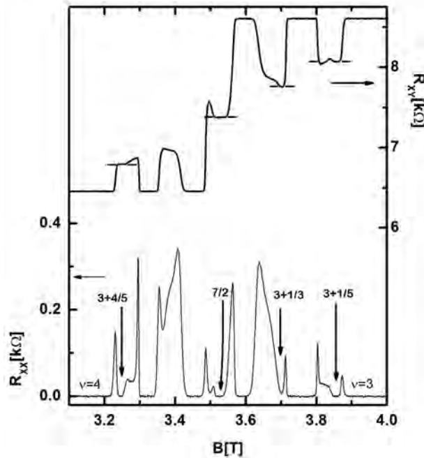
Fig. 1: Fractional quantum Hall states in the upper spin branch of the second Landau level.
