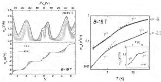
Fig. 1: Left: s_{xx} and s_{xy} as a function of the gate voltage and LL filling factor at 19 T and for several temperatures. Right: s_{xx} as a function of temperature, in a log-log scale plot, at 19 T and for several LL filling factors.
