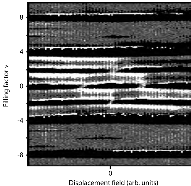
Figure 1. Layer polarization of quantum Hall states in the lowest Landau level octet in bilayer graphene. The shading scale is proportional to the difference in inverse compressibility as determined from (i) top-gate and from (ii) penetration-field capacitance. Bright white areas indicate layer polarization of the Landau levels.
