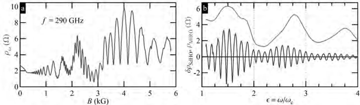
Fig. 1: (a) Resistivity \rho_\omega versus magnetic field B under microwave radiation of frequency f = 290 GHz. (b) dr_{\text{MIRO}} (top) and dr_{\text{SdHO}} (bottom) as a function of \epsilon = \omega/\omega_c .
