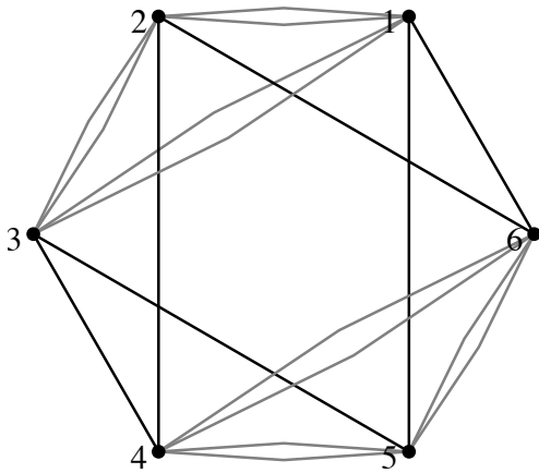
Figure 1. Sample correlation diagrams selected from (n_2, n_1, n_0) = (6, 6, 3) . G\{z_{ij}\} = S_6\{z_{12}^2 z_{13}^2 z_{15}^2 z_{16}^2 z_{23}^2 z_{24}^2 z_{26}^2 z_{34}^2 z_{35}^2 z_{45}^2 z_{46}^2 z_{56}^2\} . Here, S_6 symmetrizes the factor in curly brackets over all particles.
