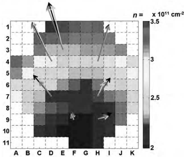
Fig. 1: Density color map of 2-inch GaAs QW wafer calibrated from dicing it into 4 \times 4 \text{ mm}^2 samples. Black arrows represent density gradients from the local density map, and the green (pink) arrows represent the density gradients using the ALR analysis method introduced here using corner (flat) contacts.
