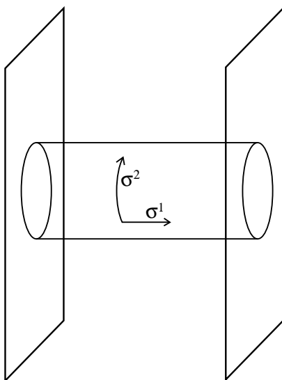
Figure 22: D-branes interacting via the tree-level exchange of a closed string.
