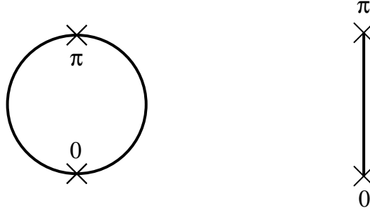
Figure 9: The orbifold S^1/Z_2 .
