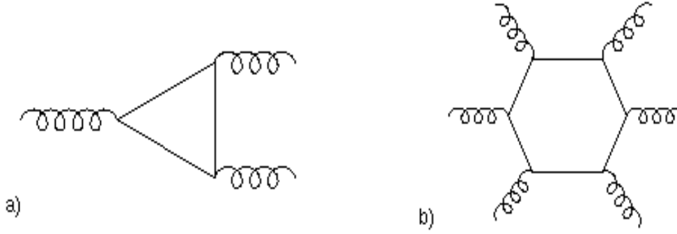
Figure 14: a) The anomalous triangle diagram in four dimensions. b) The anomalous hexagon diagram in ten dimensions.
