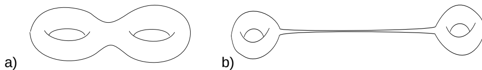
Figure 10: a) The double torus. b) The degeneration limit into two tori.
