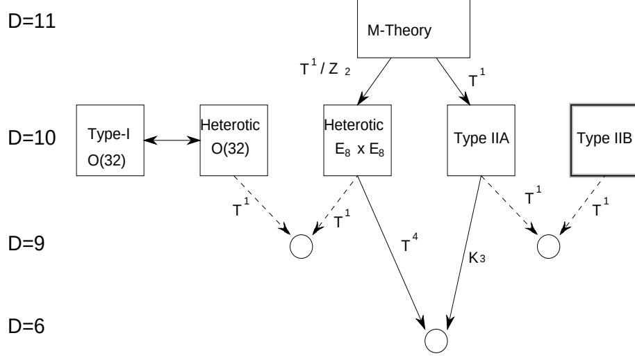
Figure 19: The web of duality symmetries between string theories. Broken lines correspond to perturbative duality connections. Type-IIB in ten dimensions is supposed to be self-dual under SL(2, \mathbb{Z}) .
