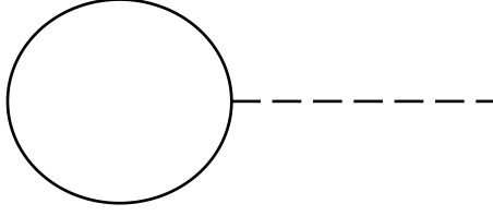
Figure 17: One-loop dilaton tadpole
