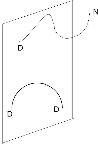
Figure 21: Open string fluctuations of a D1-brane
