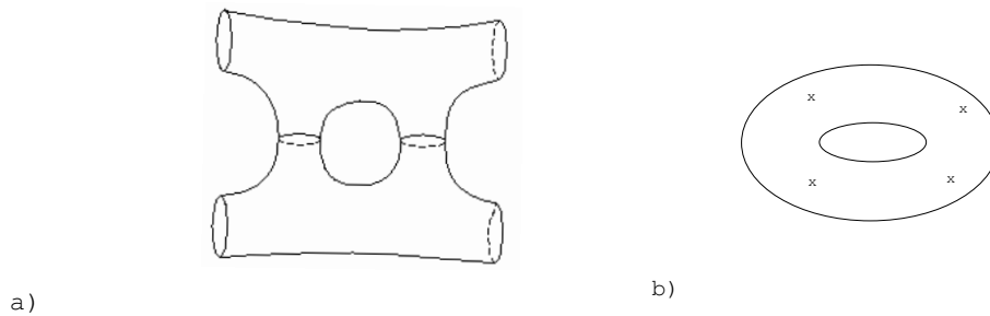
Figure 3: a) World-sheet relevant for the one-loop contribution to four-point scattering; b) Its conformal transform where the holes become punctures on a torus.
