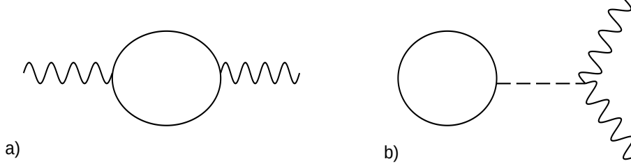
Figure 16: a) One-loop gauge coupling correction due to charged particles. b) Universal one-loop correction.
