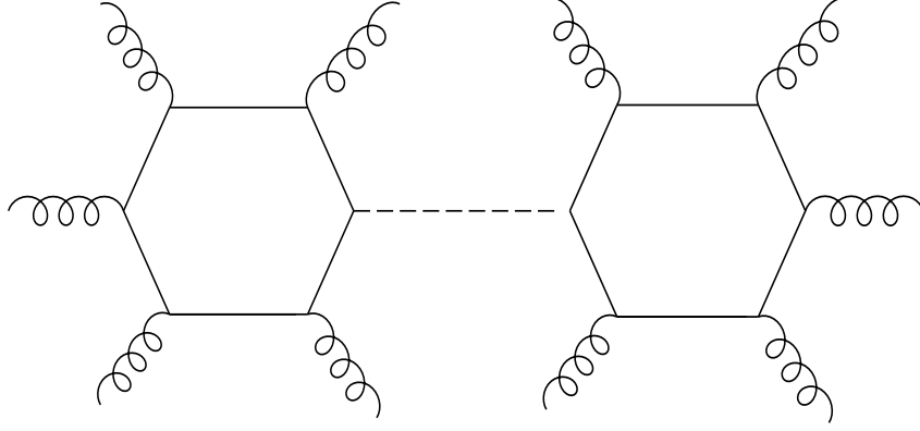
Figure 15: Two-loop diagram with physical external legs in which longitudinal modes propagate.
