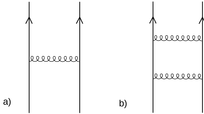
Figure 1: Gravitational interaction between two particles via graviton exchange.
