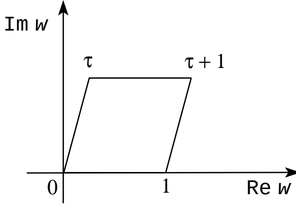
Figure 6: The torus as a quotient of the complex plane.
