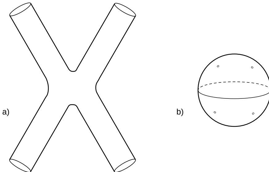
Figure 2: a) Tree closed string diagram describing four-point scattering. b) Its conformal equivalent, the four-punctured sphere
