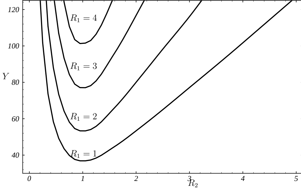
Figure 18: Plots of the universal thresholds Y(R_1, R_2) as a function of R_2 for R_1 = 1, 2, 3, 4 .
