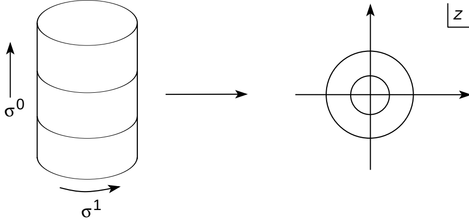
Figure 4: The map from the cylinder to the compactified complex plane
