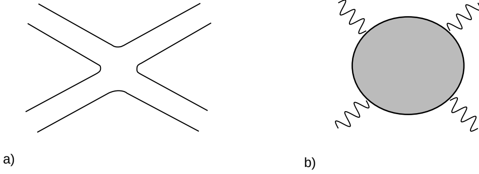
Figure 12: a) The four-point open string tree amplitude. b) Its conformal transform to a disk with four points marked on the boundary.
