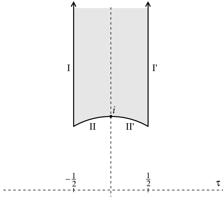
Figure 8: The moduli space of the torus.
