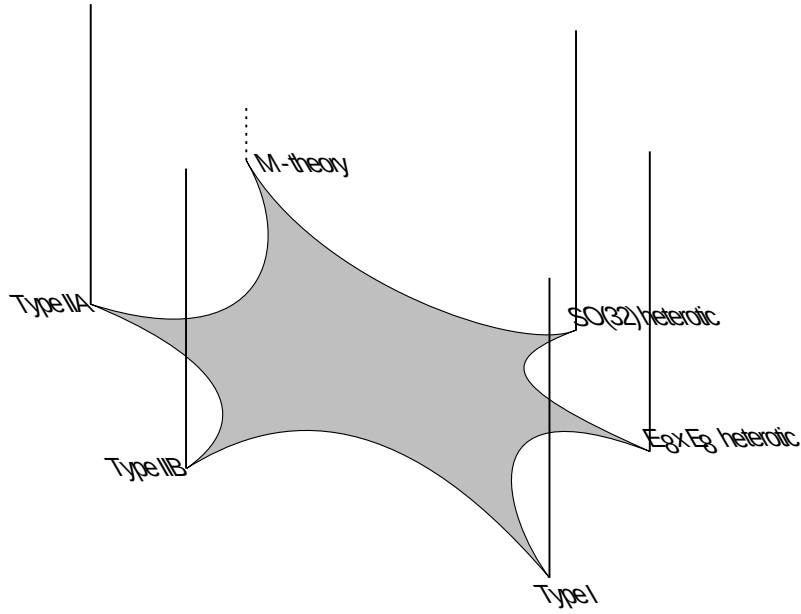
Figure 20: A unique theory and its various limits.
