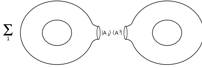
Figure 11: The Hamiltonian description of its degeneration into a pair of tori.
