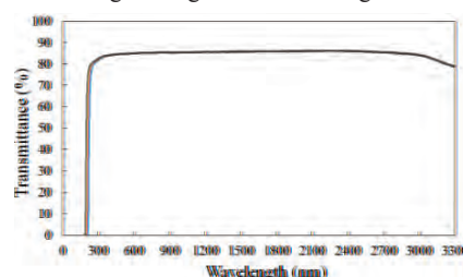
Fig.2: Optical transmittance
