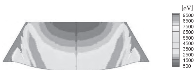
Fig. 1. Difference of nucleation energy between 3C and 6H (Substrate : 6H-SiC C-face, Growth temperature : 2300K, Growth pressure : 1Torr)
