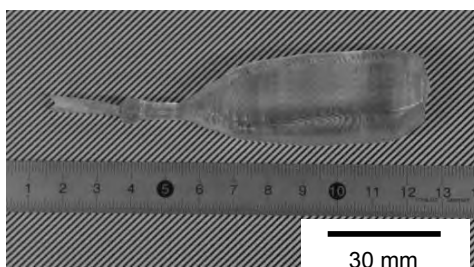
Fig.1 \text{Ca}_3\text{Ta}(\text{Ga}_{0.5}\text{Al}_{0.5})_3\text{Si}_2\text{O}_{14} single crystal grown by the Cz method
