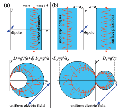
Fig. 2: Using conformal transformations for the design of nanocavities with the electromagnetic properties of infinite systems.
