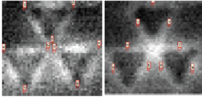
Fig. 1: Example of electron energy loss distribution of two different collective modes of a nanoantenna trimer fabricated using electron beam lithography.
