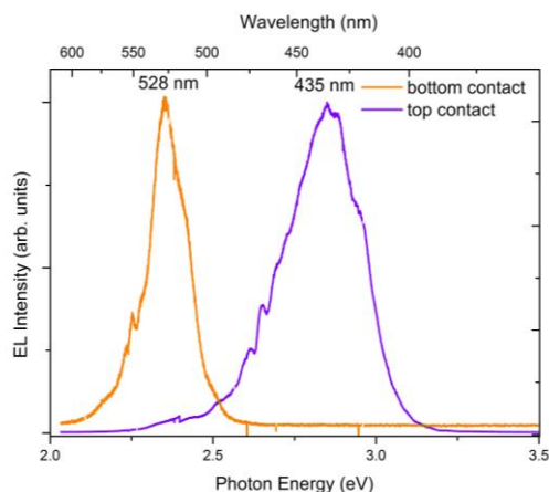
Figures show a single InGaIn/GaN nanowire LED exhibiting either blue or green emission depending on the contact position.
