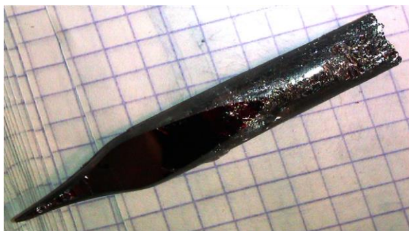
Figure 1. Bridgman grown ingot of GaSe:Cr (0.1 mass % Cr in melt).
