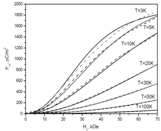
Figure 1. Dependency of polarization in \text{HoAl}_3(\text{BO}_3)_4 on H_x at different temperatures. Dotted curves are the experiment.
