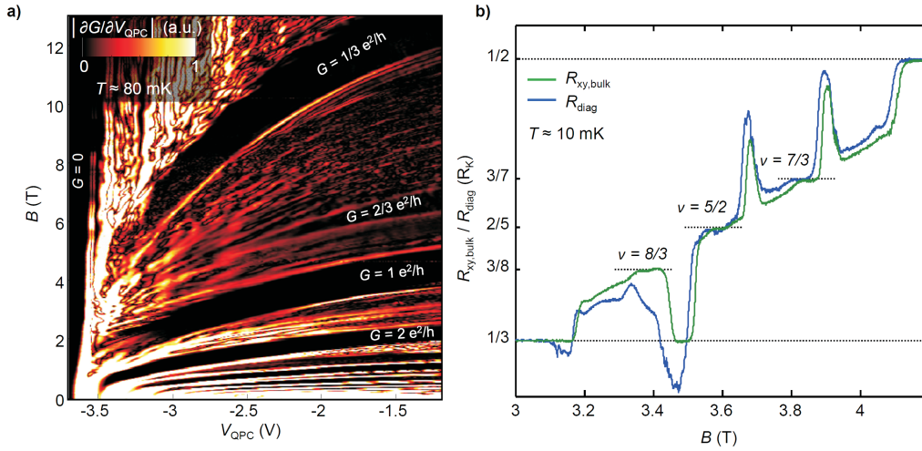
Figure 1: (a) Transconductance through a QPC as a function of the gate voltage V_{\text{QPC}} and the magnetic field B . Black regions correspond to the transmission of integer or fractional quantum Hall states through the QPC. (b) R_{\text{diag}} and R_{xy,\text{bulk}} (in multiples of R_K ) as a function of the magnetic field. The diagonal resistance across the 1.2 \mu\text{m} wide QPC reveals a fully quantized \nu = 5/2 and \nu = 7/3 states with weak backscattering at the QPC constriction.
