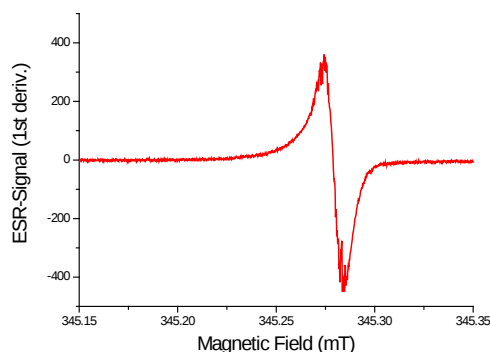
Figure 1. ESR Signal, X-band, 20 dB at-tenuation. The line width is 8.16 \mu\text{T} .
