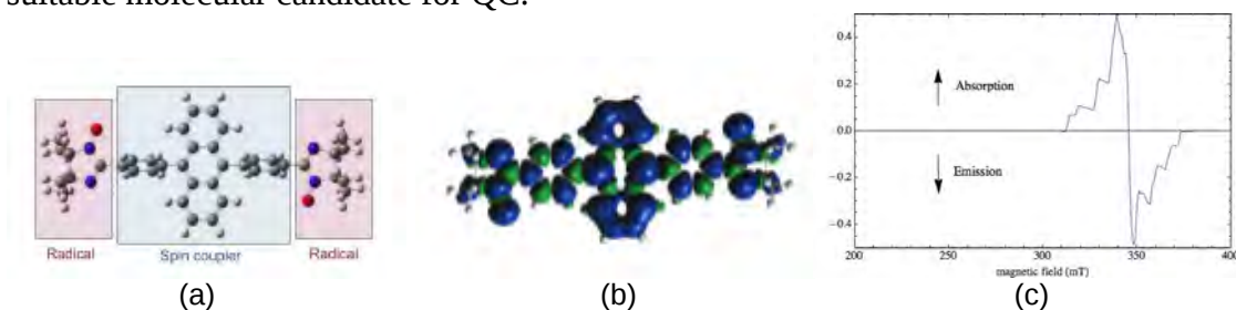
Fig.1: (a) biTTY-DPA molecule, H is in white, C in grey, O in red, and N in blue. (b) the spin density of the high spin configuration with spin up in blue and spin down in green. (c) Simulated EPR spectra of biTTY-DPA after optical excitation.
