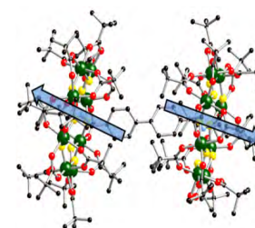
Figure 2. Structure of linked molecular qubits.
