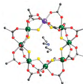
Figure 1. Structure of an anti-ferromagnetic Cr-wheel.
