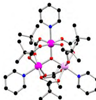
Figure 1. Representative molecular structure of [\text{Ru}_2\text{M}(\mu_3\text{-O})(\text{piv})_6(\text{py})_3] .
