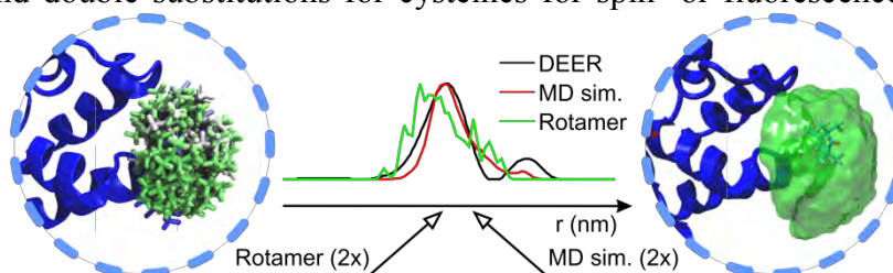
Figure 1. Experimental & simulated inter spin distance distributions.
