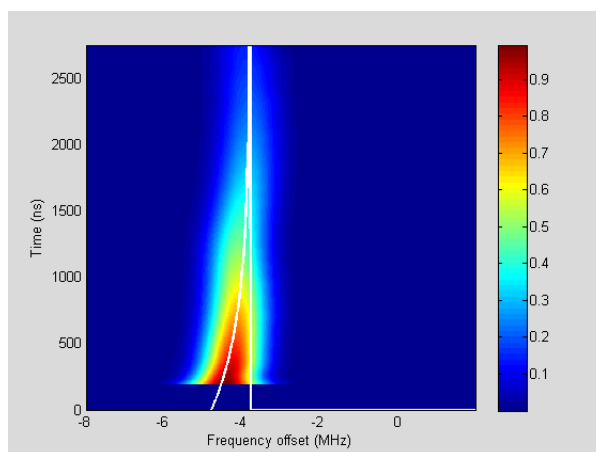
Figure 2. Time evolution of the FID-signal after a 60ns \pi/2 -pulse at t=0 . White line: Chirped FID with 1MHz shift and \tau=650 ns.
