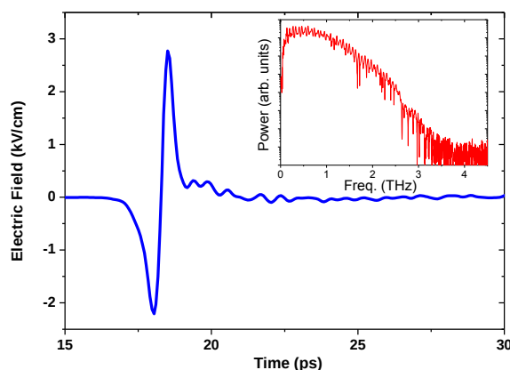
Fig. 1. Time-domain scan of the broadband terahertz radiation source. Inset shows the bandwidth of the source in the frequency domain.
