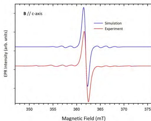
Figure 2. 15 K experimental EPR spectrum and simulation assuming Ti central hyperfine.
