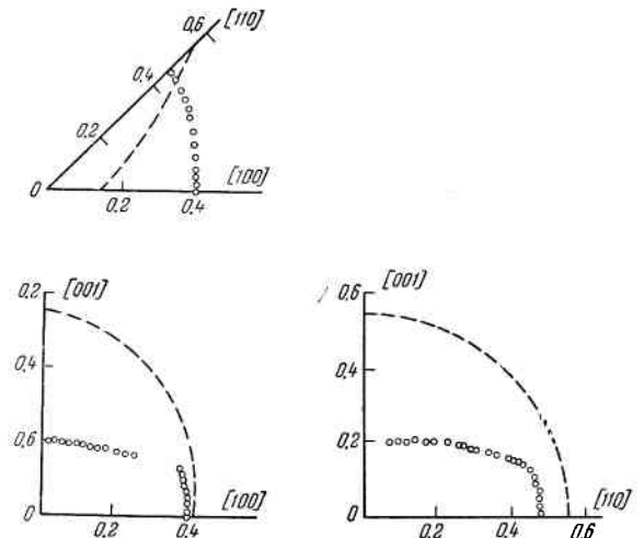
FIG. 4. Dimensions and shape of the closed Fermi surface in tin as determined by the size effect. The dashed line indicates the almost free electron model.
