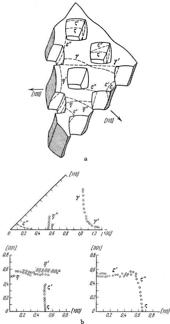
FIG. 3. a – Simplified model of the Fermi surface of the 4a zone (the shaded region is not filled with electrons), b – is the cross section determined by the size effects on the extremal orbits of this zone.
