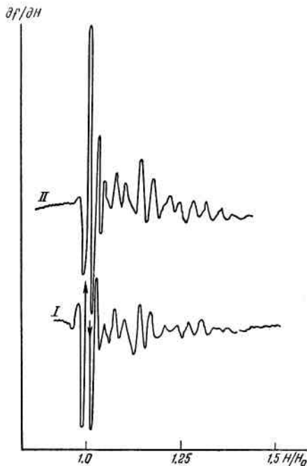
FIG. 2. Recorded lines of the size effect for n \parallel [001] , \mathbf{E} \parallel [100] . \mathbf{H} lies in the plane of the specimen and makes an angle of 14^\circ with the [010] axis (the cross section 10); curve I — d = 0.4 mm, T = 2.2^\circ\text{K} , f = 3.3 Mc; II — d = 0.6 mm, T = 3^\circ\text{K} , f = 3.7 Mc. The record of the very high maximum is cut off on curve I.
