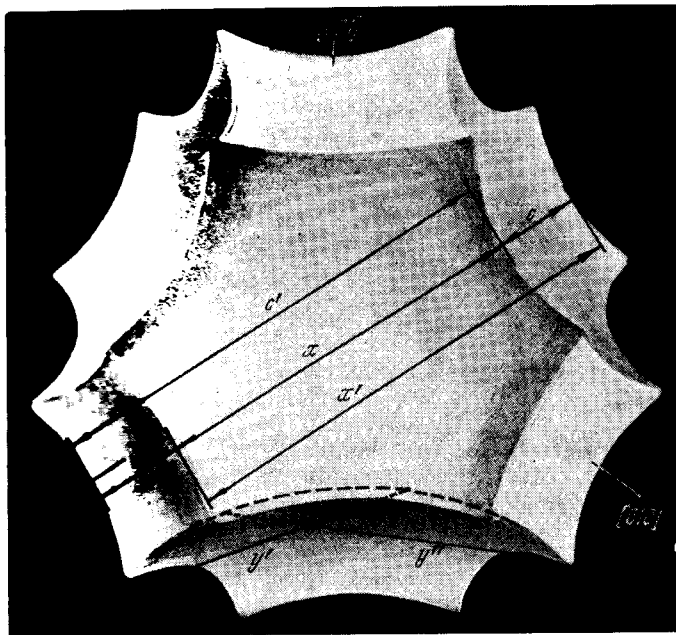
FIG. 13. View of the second zone Fermi surface from the [111] direction. Measured dimensions for H \parallel [0\bar{1}1] are indicated by arrows. Segments y' and y'' are the locations of the intersecting plane determining the corresponding lines. The dashed curve is the geometric locus of points for which (2) is fulfilled.
