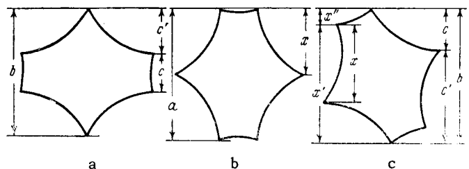
FIG. 12. Measured central cross section dimensions of the second zone Fermi surface for different normals n with a fixed field direction \mathbf{H} \parallel [011] . a – sample 2, diagram 2 (line b was not observed experimentally); b – sample 4, diagram 4; c – sample 7 (line x'' was not observed).
