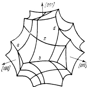
FIG. 11. Second zone Fermi surface of In on the free-electron model. Different orbits are shown for a sample with n \parallel [001] .
