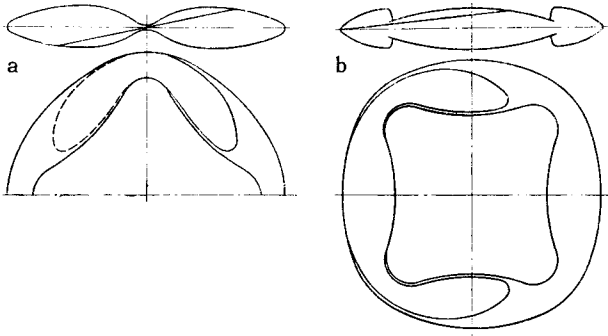
FIG. 9. Schematic drawing of f orbits—profile (from the direction of the normal \mathbf{n} ), and plane of the ring. a— f_2 orbits, \mathbf{n} \parallel [100] ; b— f_3 orbits, \mathbf{n} \parallel [110] .
