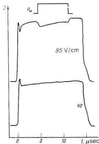
FIG. 4. Influence of microwave irradiation on the time dependence of the current flowing through the sample at different values of E ; E_\omega \approx 30 V/cm, H = 60 kOe.
