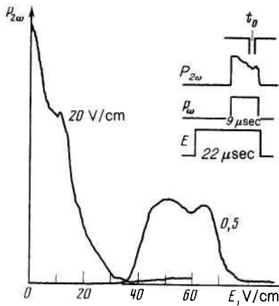
FIG. 6. Suppression of the parametric excitation of hypersound and of the harmonic generation by a constant electric field (curve at E_{\omega} = 20 V/cm); H = 45 kOe. For comparison, a plot of P_{2\omega}(E) is shown for small E_{\omega} . The inset shows the time t_0 elapsed from the start of the pulse and the instant when the power was measured.
