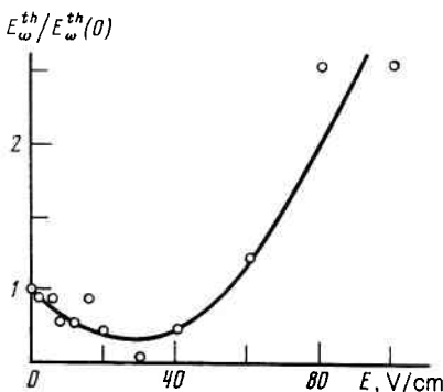
FIG. 7. Dependence of the threshold E_{\omega}^{th} on the constant field E ; H = 46 kOe.
