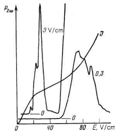
FIG. 5. Dependence of the second-harmonic power P_{2\omega} on E at various amplitudes E_\omega . Both curves were plotted for equal sensitivity of the receiving channel at the frequency 2\omega . To compare the positions of the generation channel the figure shows also the I - V characteristic; H = 60 kOe.
