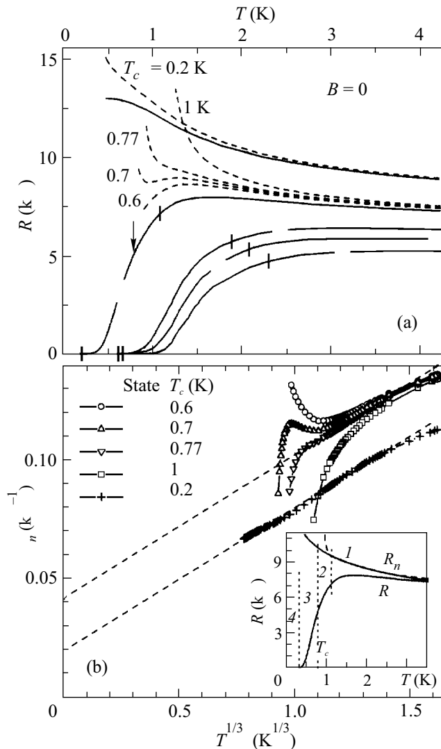
Fig.1. (a) Zero-field resistive s -transitions for several states of an amorphous \text{In-O} film. Bars frame the transition region ( 0.9R_{\text{max}} - 10^{-3}R_{\text{max}} ) on the curves R(T) . Dash curves – one for state \alpha and several, with different values of parameter T_{c0} , for state \beta – show virtual normal state resistance R_n^*(T) obtained after subtraction of the paraconductivity term calculated in accordance with Eq.(5). The selected value of T_{c0} for state \beta is shown by the arrow. (b) The dash curves from panel (a) presented as \sigma_n^* = (R_n^*)^{-1} vs T^{1/3} (form appropriated for a 3D non-Drude metal in critical region near the metal-insulator transition). Linear extrapolation cuts off the tail from the region of strong fluctuations and transforms \sigma_n^* into \sigma_n . Inset: Functions R , R_n , and R_n^* (dash line) for state \beta . About four temperature regions see text
