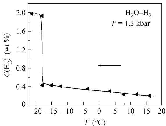
Fig. 2. Solubility of hydrogen in \text{H}_2\text{O} in the course of decreasing temperature at a pressure of 1.3 kbar.
