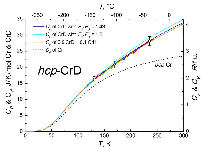
Fig. 10. Temperature dependences of the isobaric heat capacity C_p for hcp -CrD and bcc -Cr. The solid blue curve is the same as in Fig. 9. The solid cyan curve represents the sum C_V^{\text{calc}} + C_{el}^{\text{CrH}} + \Delta C_{pV}^{\text{CrH}} , where C_V^{\text{calc}} is calculated using g_{\text{opt}}^{\text{CrD}}(E) = 1.51g_{\text{opt}}^{\text{CrH}}(E \cdot 1.51) . The solid orange curve shows the heat capacity of a mixture of 90% CrD + 10% CrH. (For interpretation of the references to color in this figure legend, the reader is referred to the Web version of this article.)
