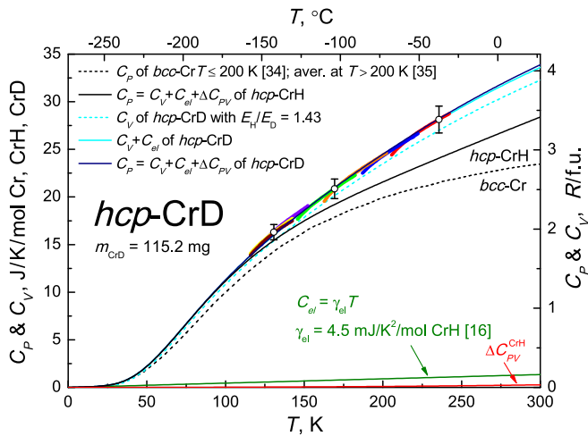
Fig. 9. Segments of thick colored curves represent the temperature dependence of the isobaric heat capacity C_p^{\text{exp}} of hcp -CrD measured at a heating rate of 20 K/min. Some experimental points of C_p^{\text{exp}} are plotted as open black circles intersected by vertical bars indicating the experimental error 5%. The solid blue curve shows the C_p^{\text{calc}}(T) dependence of hcp -CrD calculated in this paper as the sum of the phonon heat capacity C_V^{\text{calc}} of hcp -CrD (dashed cyan curve), the electronic heat capacity C_{el}^{\text{CrH}} (solid olive line at the bottom of the Figure) and the difference \Delta C_{pV}^{\text{CrH}} = C_p(T) - C_V(T) (solid red curve at the bottom of the Figure). Also shown are the sum C_V^{\text{calc}} + C_{el}^{\text{CrH}} for hcp -CrD (solid cyan curve), C_p^{\text{exp}} for hcp -CrH (solid black curve), and the experimental C_p for bcc -Cr reported in Refs. [34,35] (dashed black curve). The temperature dependences of C_p and C_V for CrD and C_p for CrH can also be found in digital format in the Supplementary file “Cp and Cv for CrH and CrD.dat”, and \Delta C_{pV}^{\text{CrH}} in the file “Delta CpV for CrH.DAT”. (For interpretation of the references to color in this figure legend, the reader is referred to the Web version of this article.)
