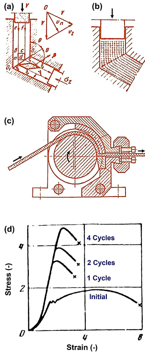
Figure 7. (a) Principles of equal-channel angular pressing (extrusion) developed by Segal et al. [20]. (b) Experimental visualization of simple shear in equal-channel angular pressing by Moiré fringes and coordinate grids [20]. (c) Combination of equal-channel angular pressing with conform developed in Minsk [86]. (d) Stress-strain curves for iron processed by equal-channel angular pressing, showing combination of high strength and good ductility (units for X and Y axes were not given in paper, but it seems each unit in X and Y axes roughly correspond to strain of 2-3% and stress of 200-250 MPa, respectively) [20].
