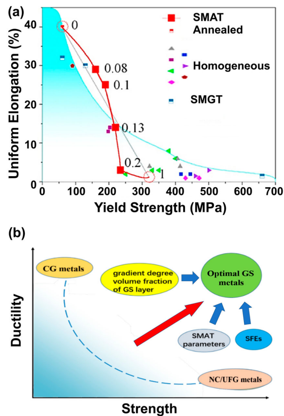
Figure 37. (a) Strength and ductility of gradient-structured copper processed by surface mechanical attrition treatment (SMAT) and surface mechanical grinding treatment (SMGT) compared with copper samples with homogenous structure [725]. (b) Basic factors affecting correlation between strength and ductility of gradient-structured materials [711,725,741–743].
