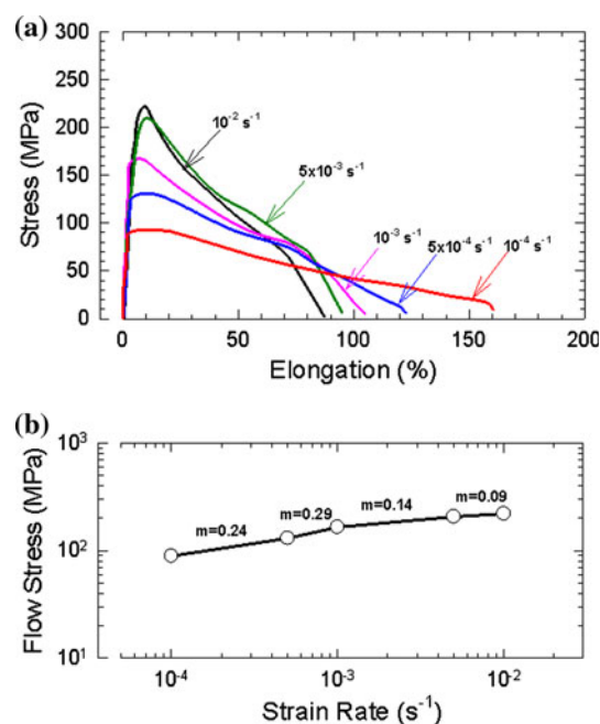
Fig. 2 a Effect of strain rate on the true stress–strain curves and b the variation of flow stress with strain rate and the values of the strain rate sensitivity, m , for the Al-30 wt% Zn alloy processed by HPT
