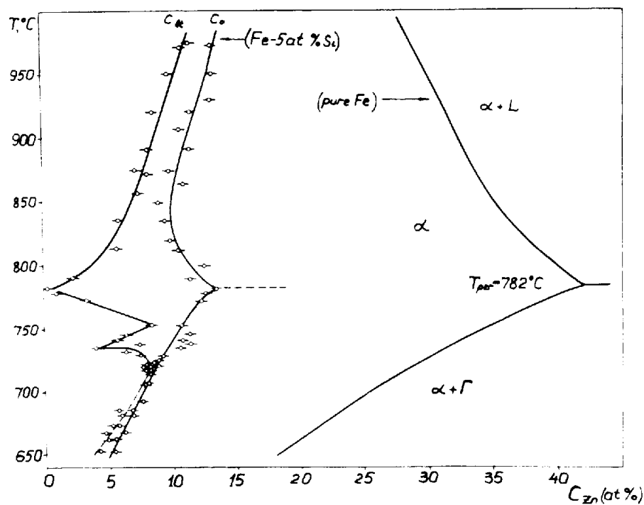
Fig. 5. Thermal dependences of c_{B1} and c_0 in the Fe-5at%Si alloy. The zinc concentration is plotted on the x-axis. The line of the solubility limit of zinc in pure iron is also displayed (solidus and solvent line).
