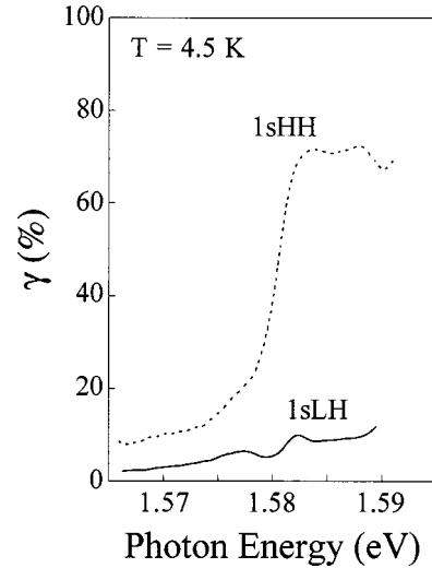
FIG. 5. Ratio \gamma=|\sigma^+ - \sigma^-|/|\sigma^+ + \sigma^-| between the photoluminescence intensities \sigma^+ and \sigma^- at T=4.5 K reported in Fig. 4 (the polarization of the exciting light is \sigma^+ ). The full (dashed) line refers to the case of resonant excitation of the 1s ground state of the light-hole (heavy-hole) exciton.
