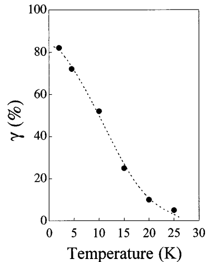
FIG. 6. The ratio \gamma=|\sigma^+ - \sigma^-|/|\sigma^+ + \sigma^-| between the photoluminescence intensities \sigma^+ and \sigma^- , evaluated at the T -band peak energy for the case of resonant excitation of the 1s HH exciton ground state, is reported as a function of temperature.
