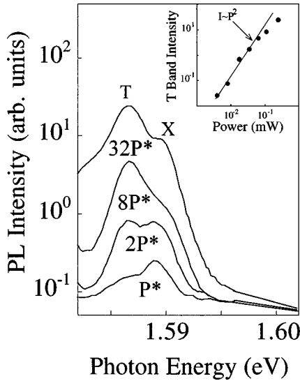
FIG. 3. Photoluminescence spectra at T=11 K for different exciting power density ( P^*=W\text{ cm}^{-2} ). The peak intensity of the T band as a function of the excitation power is reported in the inset (the full line corresponds to a quadratic dependence of intensity on power).
